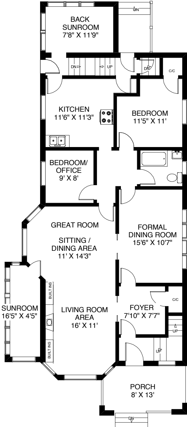
CEILING HT 9' MAIN FLOOR APPROXIMATELY 1,525 SQ FT
