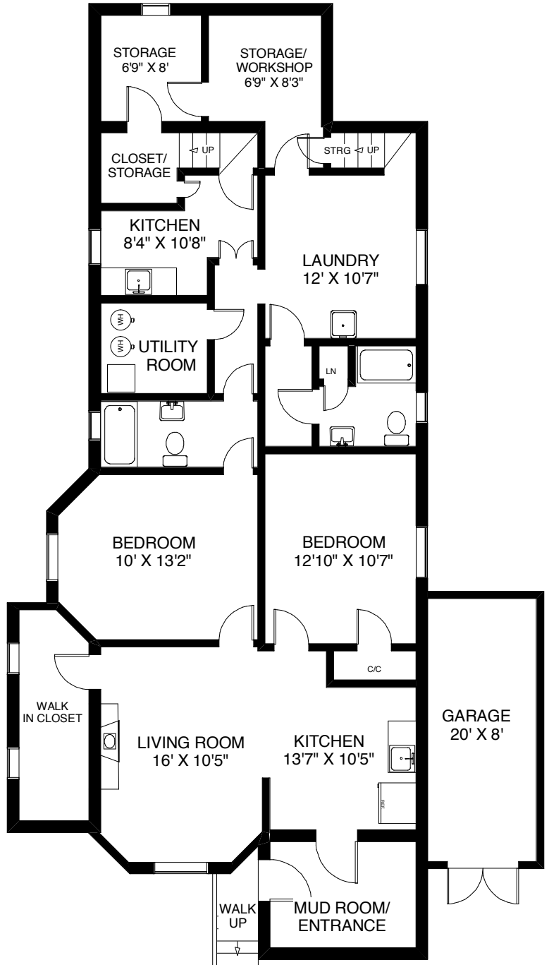
LOWER FLOOR APPROXIMATELY 1,700 SQ FT
