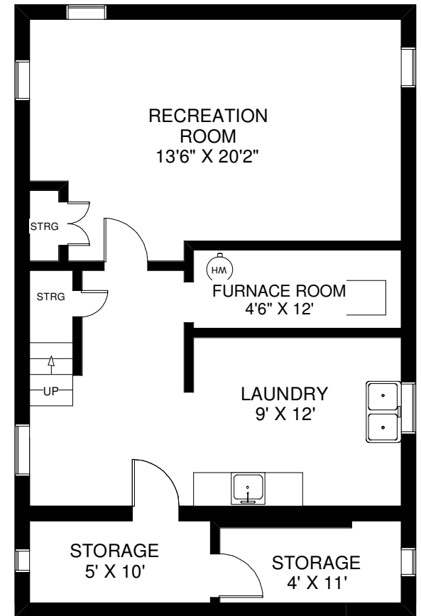
CEILING HT 6'8" LOWER FLOOR APPROXIMATELY 790 SQ FT
